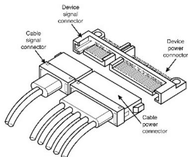
Figure 3 Attaching SATA cabling
